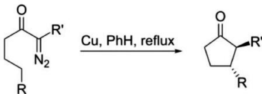
Carbene intramolecular reaction
